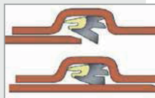
DIN-Lock-Dichtring
